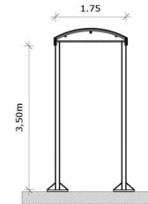
CORTE:Toldo C
